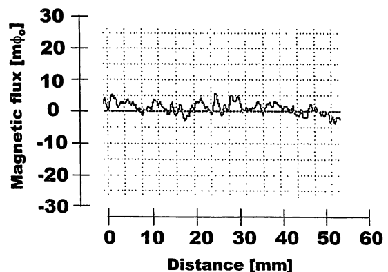
Fig. 4. Signal trace of the blank sample. The peak to peak value of the background signal is about 7 m\phi_0 .
