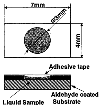
Fig. 2. Schematic drawing of the sample carrier. The size of the glass slide is 7 mm x 4 mm x 0.9mm. It has a hole of 3mm in diameter. After filling the hole with a liquid sample, it was covered with an adhesive tape.
