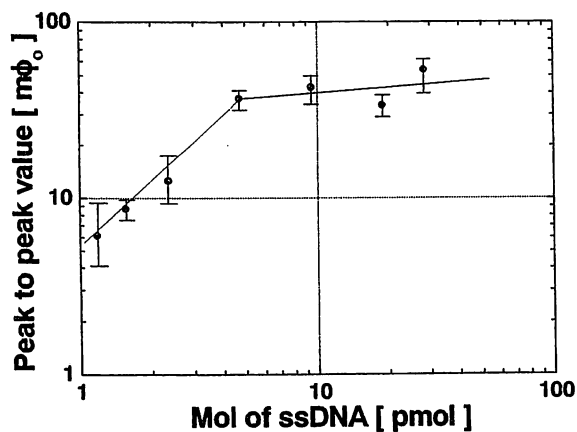
Fig.8. Magnetic signal v.s. mol of sample DNA. Horizontal axis shows the number of sample DNA applied to the probe DNA. Signal shows saturation at about 5 pmol of DNA.
