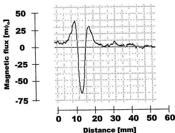
Fig. 5. Typical signal trace of a liquid sample with particles. This sample contains 0.73 pmol of nanoparticles.
