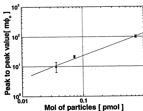
Fig. 6. Magnetic signal v.s. number of particles. Volume of the sample is 4 \mu\text{l} . The signal is almost proportional to the number of the particles.
